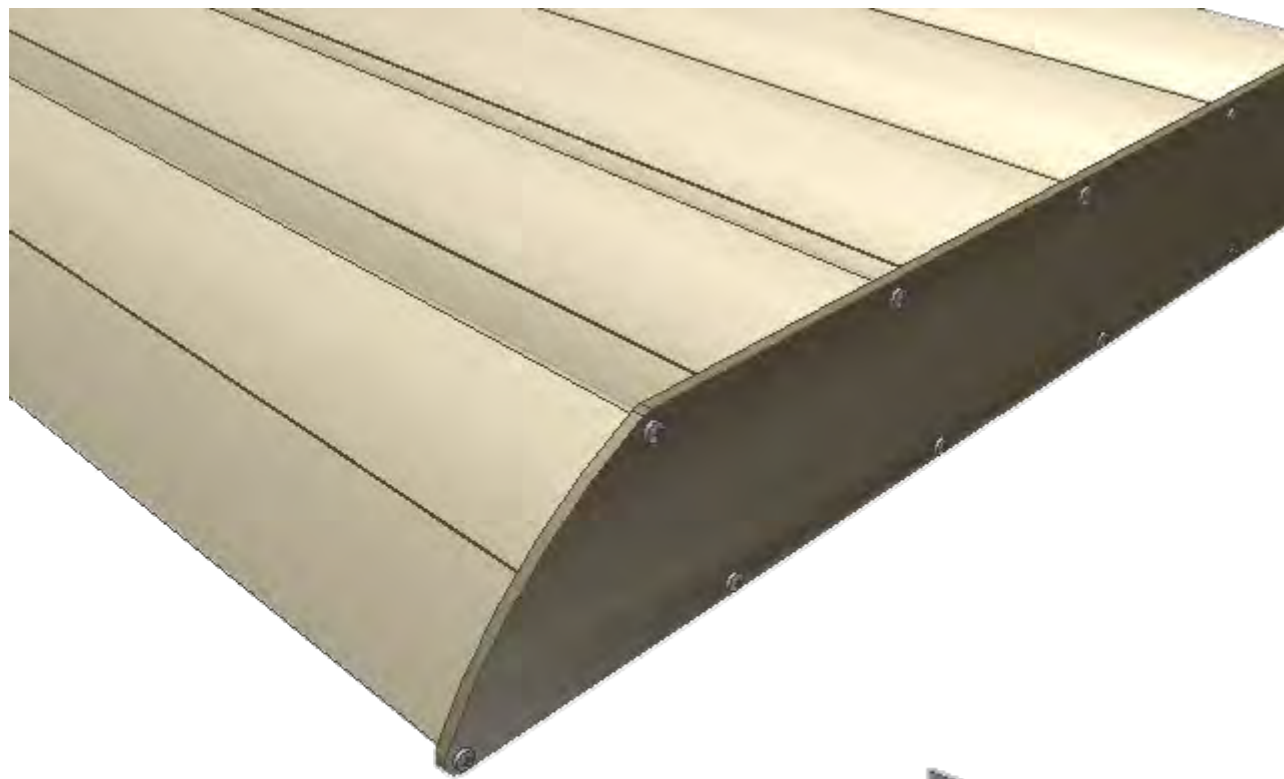
Enlarged Front Corner Detail
